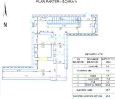
PLAN PARTER - SCARA A
